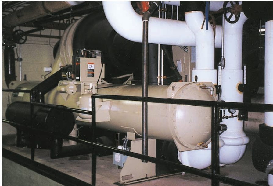
This 500-ton chiller, installed for a paper mill application, provides constant, year-round temperature and humidity control for the mill's plant and offices.
