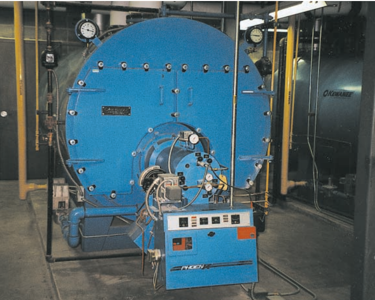
One of two hot water boilers used at a school where temperature and humidity are major concerns.
